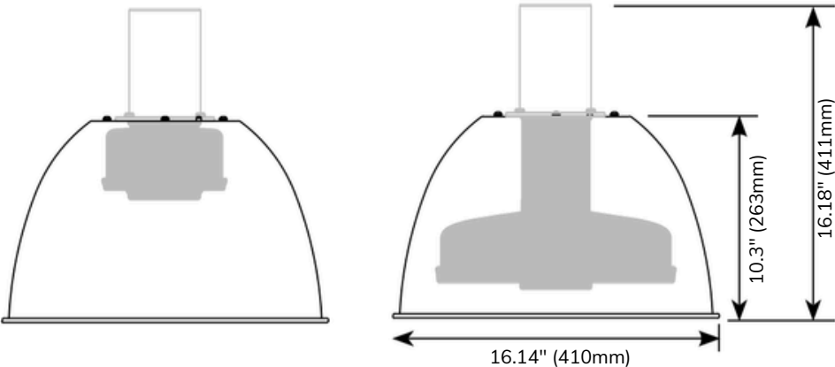
16" Prismatic Reflector shown with OEO Super Hybrid 28W to 45W LED Lamp
