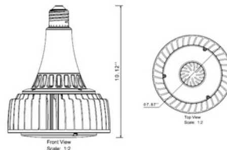
MODEL: EZ-LED-HO-U-P-4K WEIGHT: 3.13 LBS
