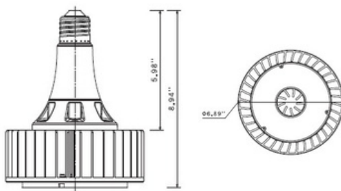
MODEL: EZ-LED-HO-D-P-5K WEIGHT: 2.3 LBS
