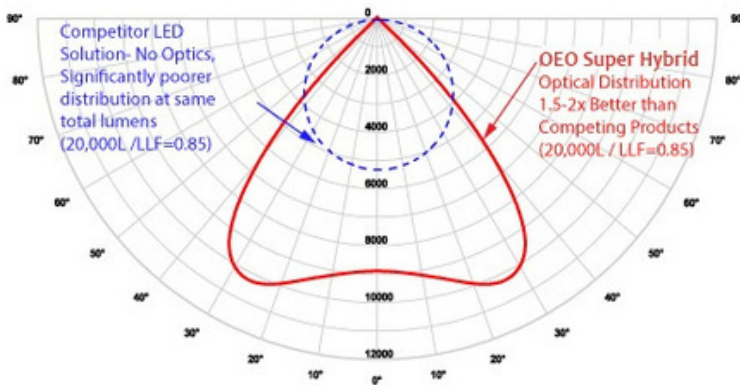
Polar Curve
