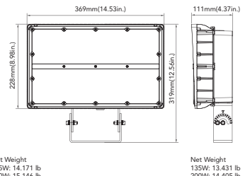
135W&200W(Yoke Mount)
