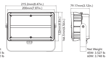
45W&60W(Trunion Mount)
