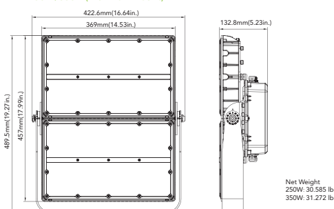
250W/350W(Trunion Mount)
