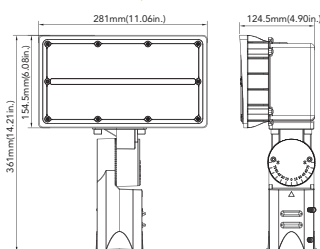
250W/350W(Trunion Mount)
